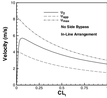
Fig. 4 Effect of top bypass on average velocities.
